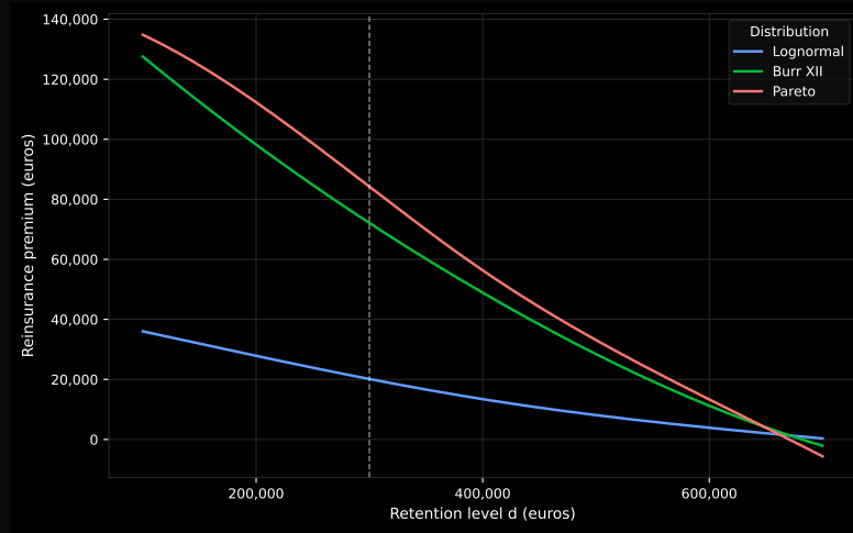
Figure 9: Reinsurance premium (110% of expected ceded loss) as a function of the retention level d .
