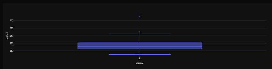
Figure 2: inhomogeneous process
