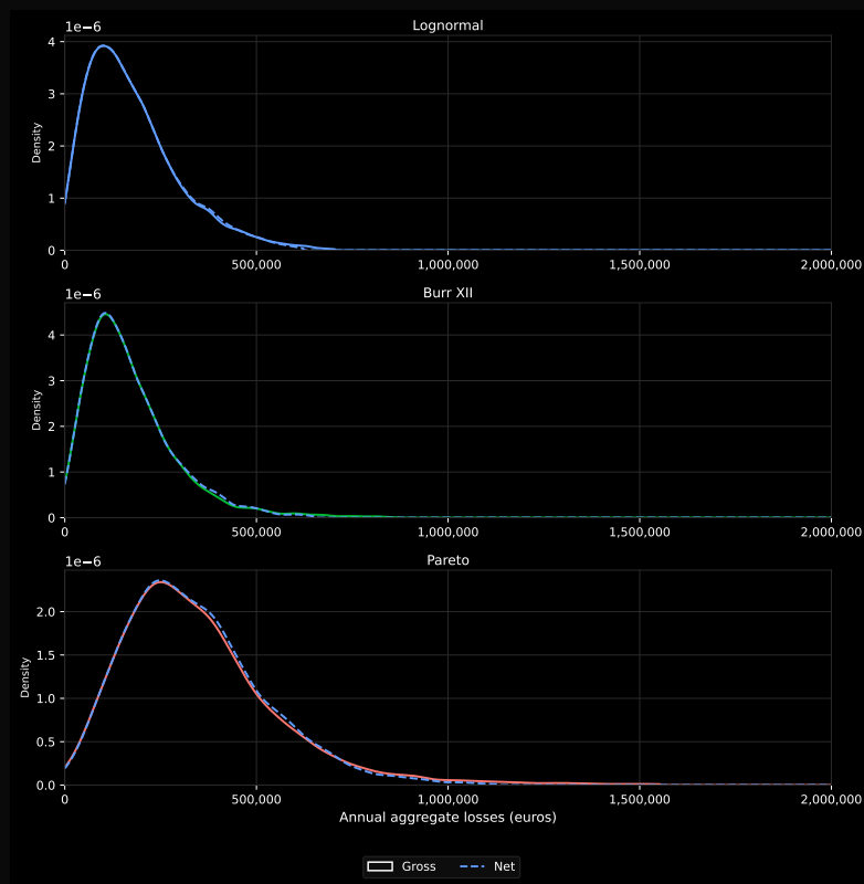
Figure 7: Gross vs. net aggregate loss distributions under the three severity assumptions.
