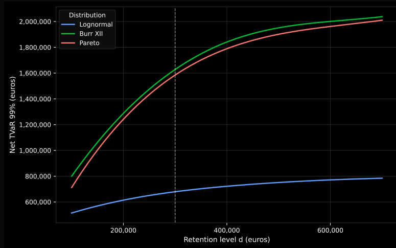
Figure 8: Net TVaR 99 as a function of the retention level d . The vertical dashed line marks the baseline d = 300,000 €.
