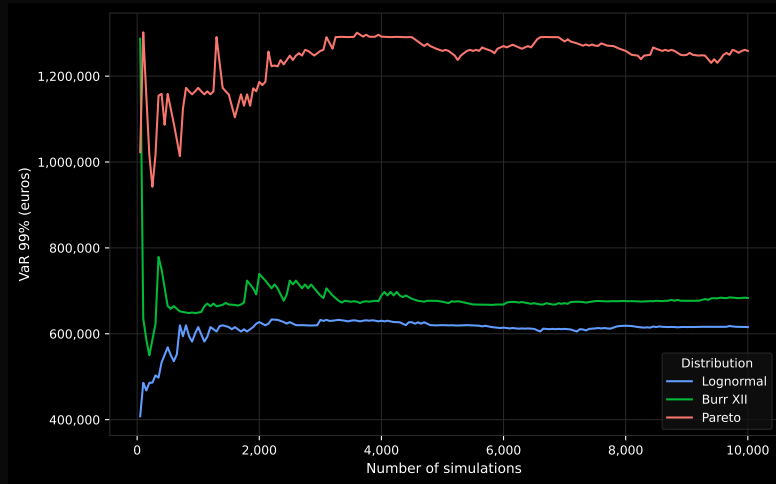
Figure 4: Convergence of the 99% VaR estimator as a function of the number of Monte Carlo replications.
