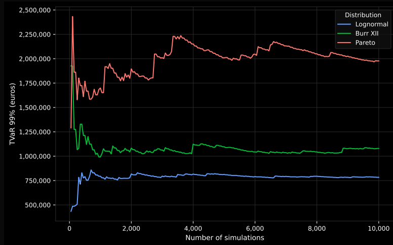
Figure 5: Convergence of the 99% TVaR estimator as a function of the number of Monte Carlo replications.
